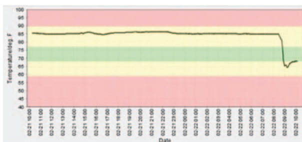
Figure 16. Effect of adding blanking panel to rack of high-performance servers.
