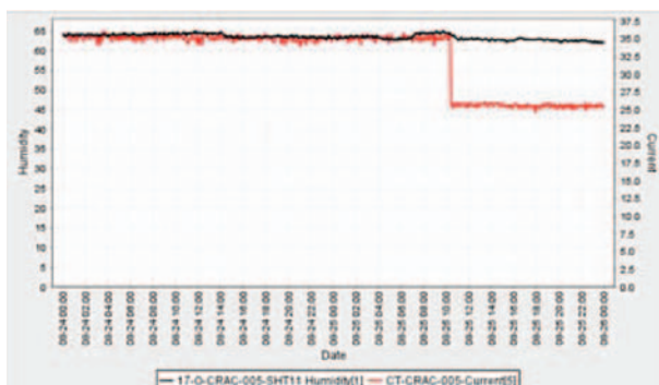
Figure 15. Effect of humidification control set to “off.”
