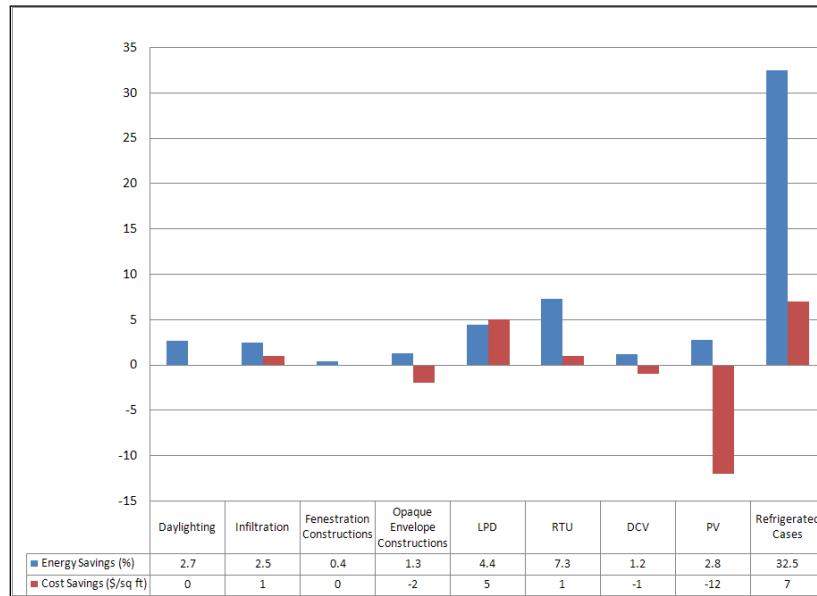
Figure 7. EDM Cost Effectiveness Breakdown for Miami Grocery
