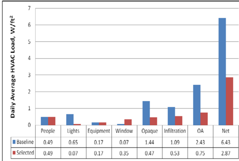
Figure 3. Average Weekday HVAC Loads for Minneapolis During January
